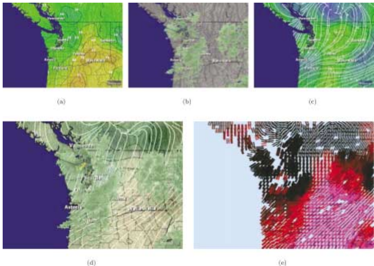
Fig. 11. Example multidimensional visualizations: (a) standard visualization of temperature with color (dark green for cooler to yellow for warmer); (b) standard visualization of precipitation with Doppler radar (green for light rainfall to red for heavy rainfall); (c) standard visualization of wind direction with directed contours and wind speed with color (dark blue for low winds to bright green for high winds); (d) a combination of three individual visualizations to form a single, multidimensional image; (e) a nonphotorealistic visualization with simulated paint strokes that vary their color, coverage, orientation, and size to visualize the same data.
